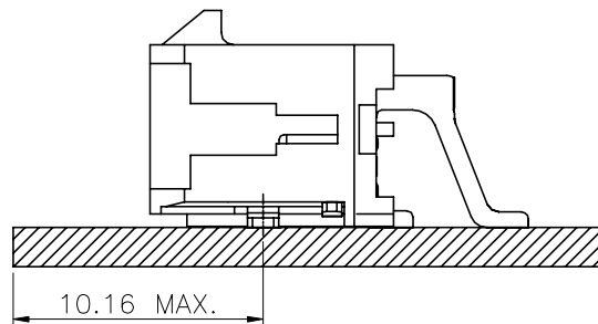
LOCATION DETAIL
